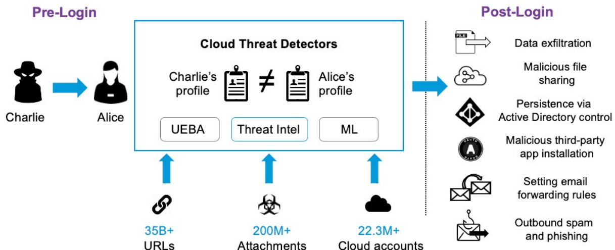
Figure 1: CASB compromised account detection.
